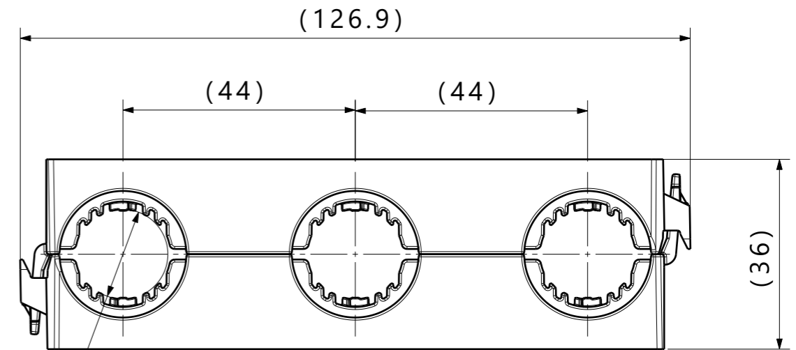
Assembled example front view
